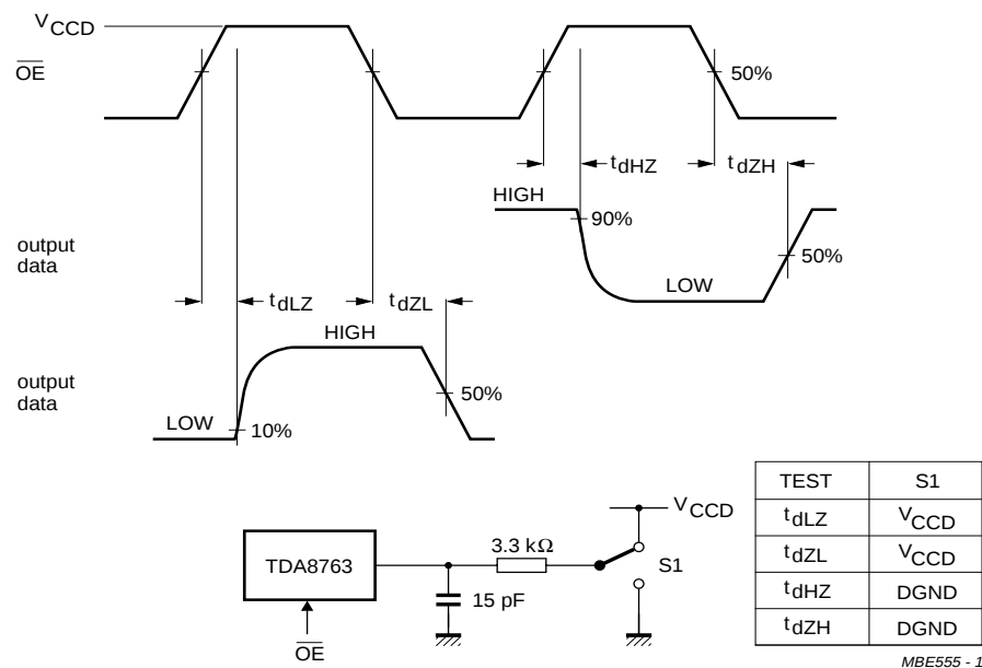
Fig.5 Timing diagram and test conditions of 3-state output delay time.
